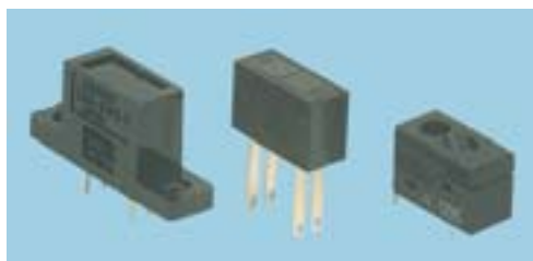
121-6966 H=15.9, W=25.4, D=6.35 121-6965 H=18, W=25.4, D=6.35 121-6967 H=17.7, W=13, D=5.7 (overall) 117-3628 H=15.6, W=13, D=5.7 (overall) 117-3632 H=11, W=14.1 (overall), D=6
